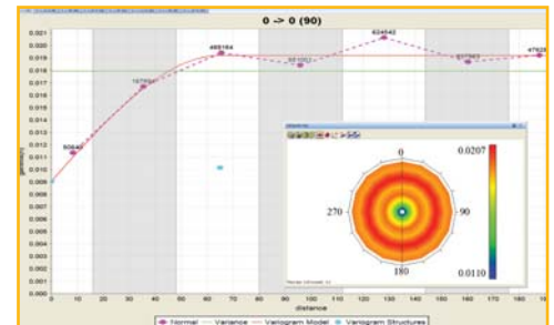
Improved presentation of variogram maps.
