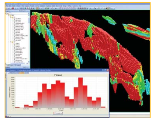
Viewing a GEMS block model in Surpac with enhanced Geostatistics.
